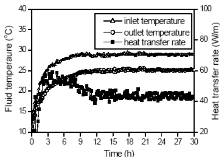
Figure 9b. Heat injection (inlet fluid temperature: 28.9 °C)
