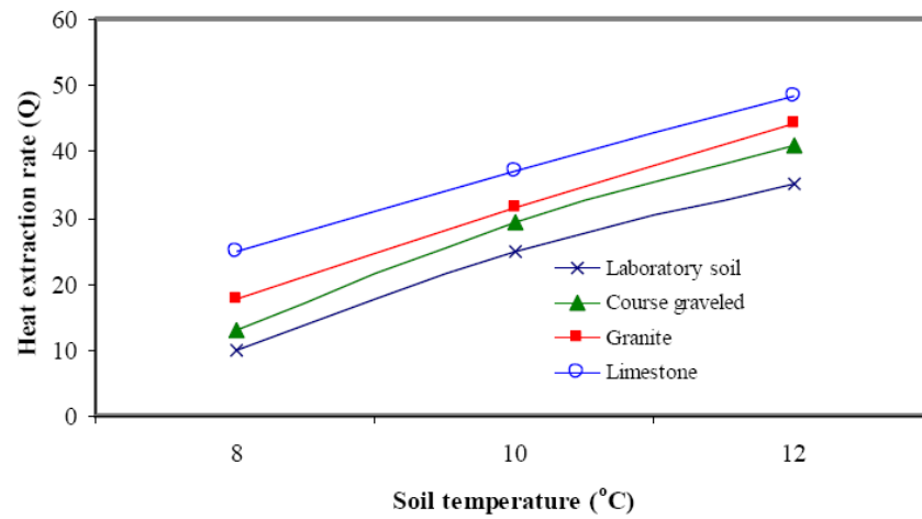
Figure 27. Heat extraction rate for 4 types of soils.
