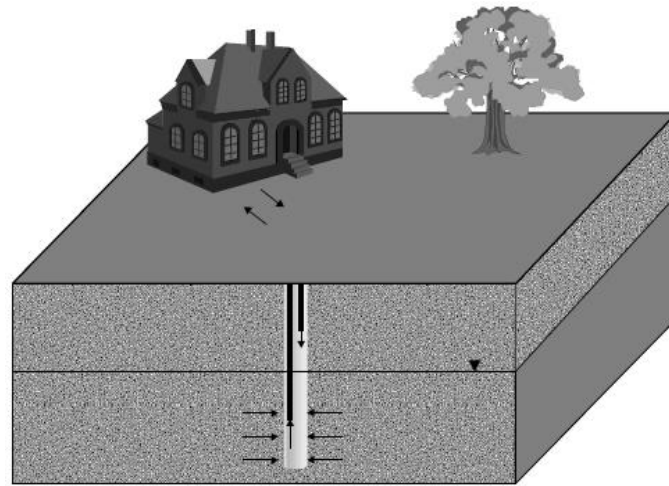
Figure 14. A schematic of a standing column well system.
