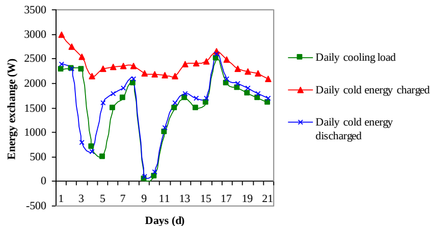
Figure 31. Simulation results in summer.
