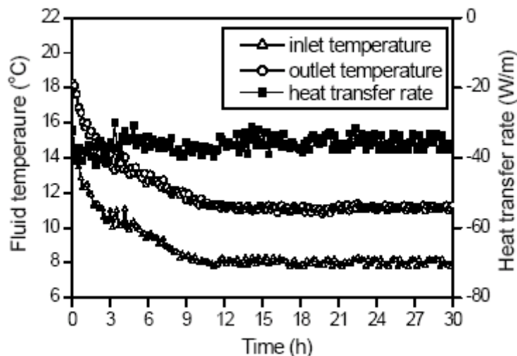
Figure 9a. Heat extraction (inlet fluid temperature: 8.0 °C).
