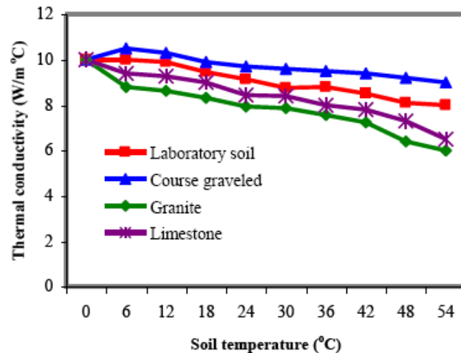
Figure 25. Comparison of thermal conductivity for different soils.
