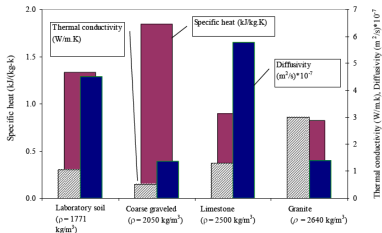
Figure 26. Thermal properties for different soils.
