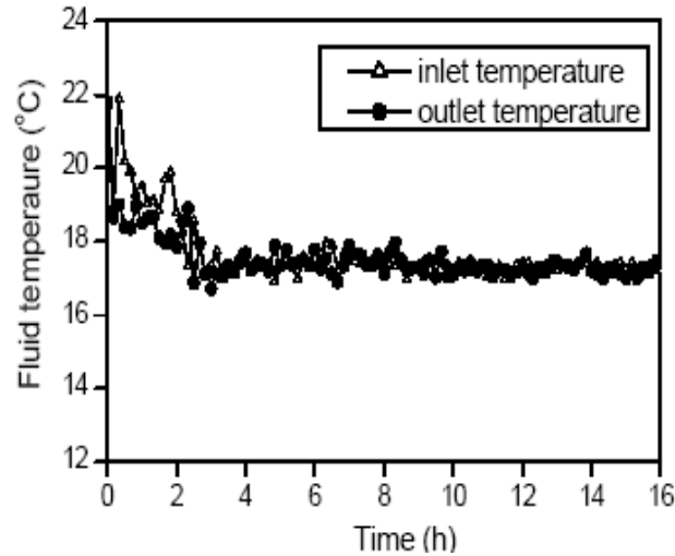
Figure 7. Test results of the natural ground temperature.
