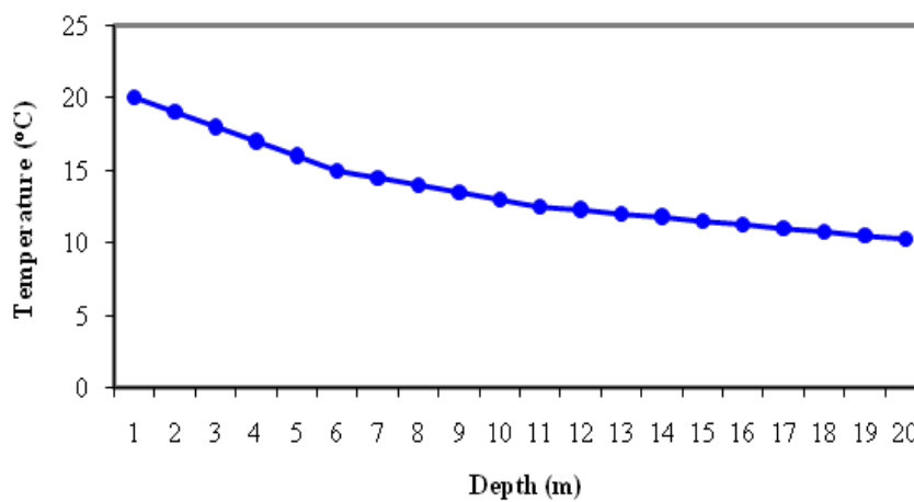
Figure 28. Variation of soil temperature ground depth.
