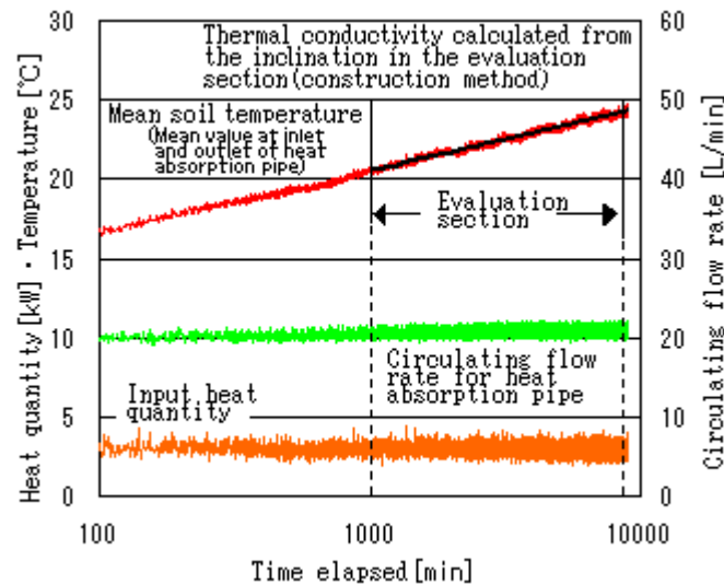
Figure 21. Thermo response test.
